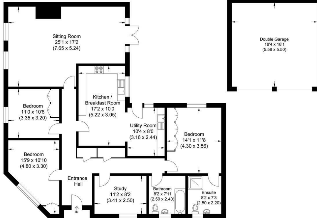
Ground Floor
